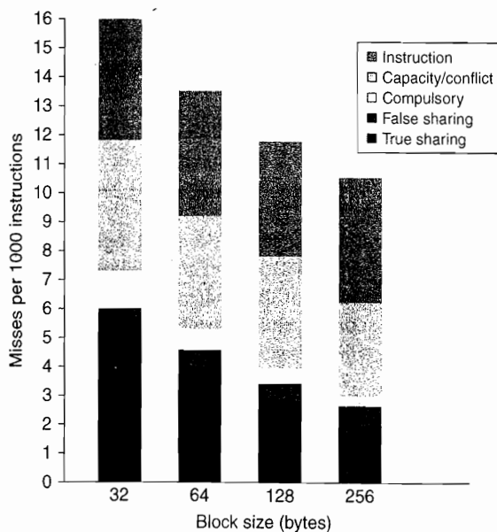
Figure 5.15 The number of misses per 1000 instructions drops steadily as the block size of the L3 cache is increased, making a good case for an L3 block size of at least 128 bytes. The L3 cache is 2 MB, two-way set associative.
