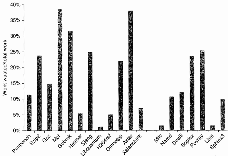
Figure 3.42 The amount of “wasted work” is plotted by taking the ratio of dispatched micro-ops that do not graduate to all dispatched micro-ops. For example, the ratio is 25% for sjeng , meaning that 25% of the dispatched and executed micro-ops are thrown away. The data in this section were collected by Professor Lu Peng and Ph.D. student Ying Zhang, both of Louisiana State University.
