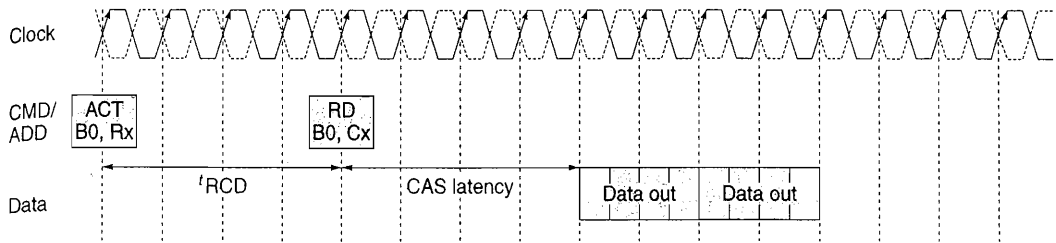
Figure 2.31 DDR2 SDRAM timing diagram.
