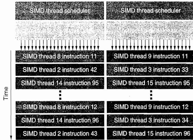
Figure 4.19 Block Diagram of Fermi's Dual SIMD Thread Scheduler. Compare this design to the single SIMD Thread Design in Figure 4.16.
