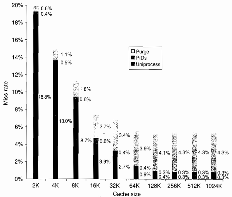
Figure B.16 Miss rate versus virtually addressed cache size of a program measured three ways: without process switches (uniprocess), with process switches using a process-identifier tag (PID), and with process switches but without PIDs (purge). PIDs increase the uniprocess absolute miss rate by 0.3% to 0.6% and save 0.6% to 4.3% over purging. Agarwal [1987] collected these statistics for the Ultrix operating system running on a VAX, assuming direct-mapped caches with a block size of 16 bytes. Note that the miss rate goes up from 128K to 256K. Such nonintuitive behavior can occur in caches because changing size changes the mapping of memory blocks onto cache blocks, which can change the conflict miss rate.
